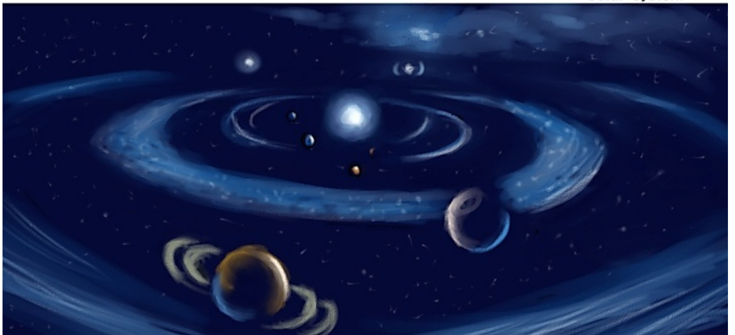
Solar System
