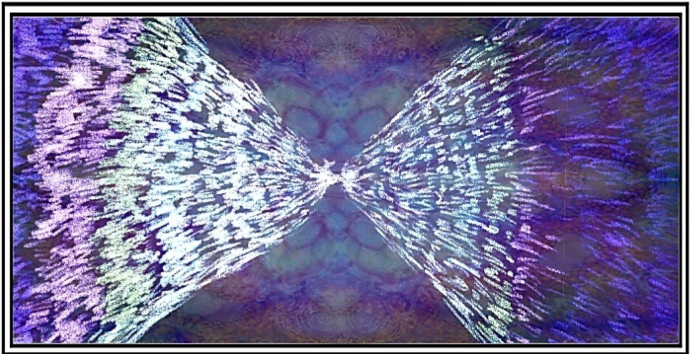
The Galaxies
