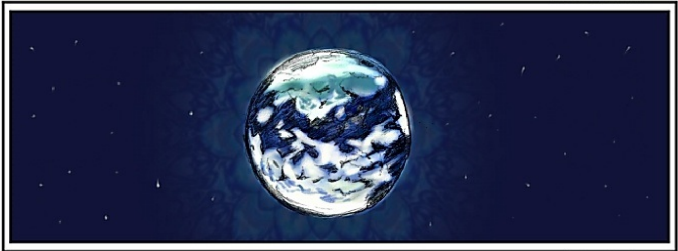
Solar System
