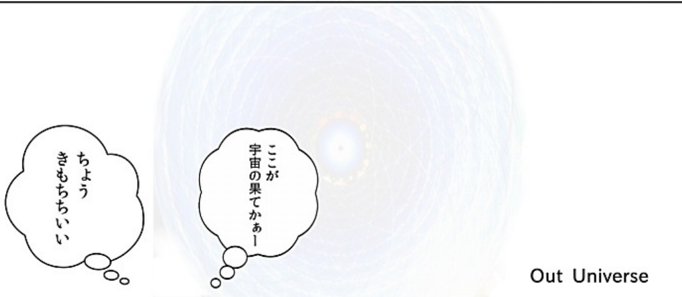
The Galaxies
